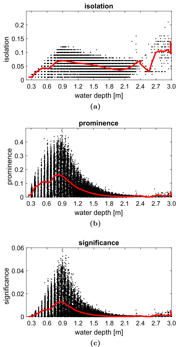
Fig. 9 Results of evaluation of optimal start depth for full-waveform stacking filtering: a isolation, b prominence, and c significance as a function of their water depth. The black points are the single values, and the red line presents the mean trend. The vertical stripe pattern in the shallow water depths (0.3–0.9 m) is caused by the sample time interval (= resolution in laser beam direction of approximately of 6.5 cm) in the full-waveform data. At greater water depths, this effect is considerably weakened by the effect of the obliquely incident laser beam
