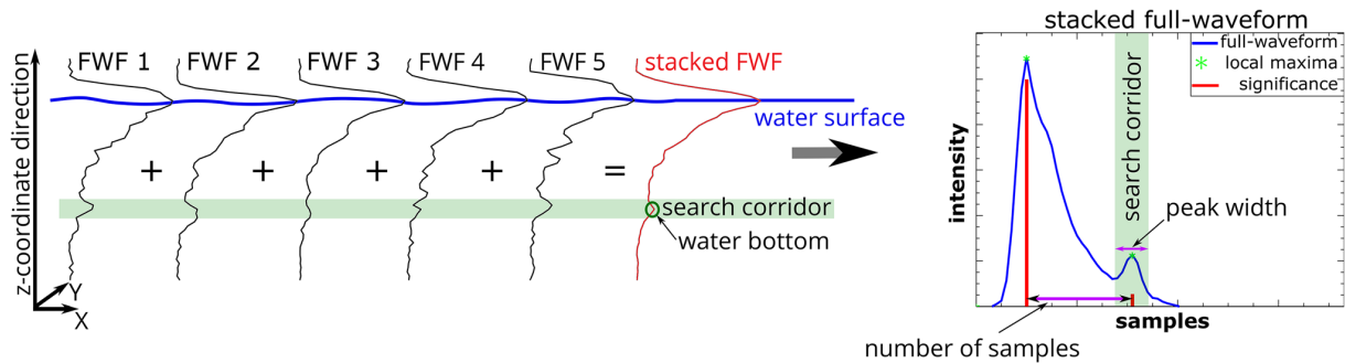
Fig. 6 Basic principle of full-waveform stacking applied to ALB pulse echo waveforms. The green marked area corresponds to the reduced search corridor for water bottom echoes in the original full-waveforms (black), based on the analysis of the stacked full-waveform (red)
