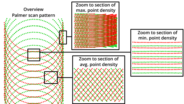
Figure 2: Schematic Palmer scan pattern (adapted from RIEGL Ri-Parameter software) showing the heterogeneous point density. Green points = forward look and red points = backward look.
