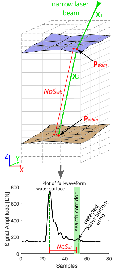
Figure 19: Detection of weak water bottom echoes in individual full-waveforms by using ortho full-waveform analysis results (initial water bottom model).
