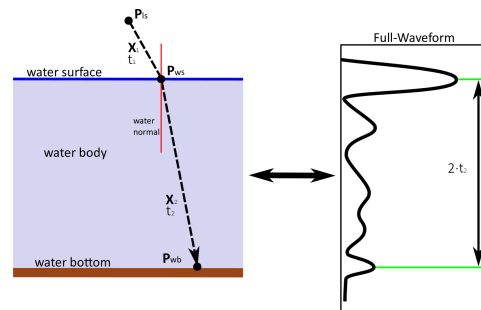
Figure 9. Schematic illustration of water bottom point calculation.
