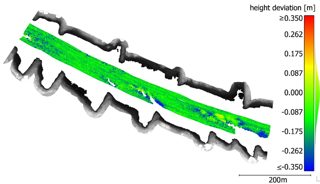
Fig. 14 Elbe 3: Height deviations between ES points and FWSP points. The compared points are colour-coded corresponding to their deviation. FWSP points with positive height deviations are estimated as deep, and points with negative height deviations are estimated as high
