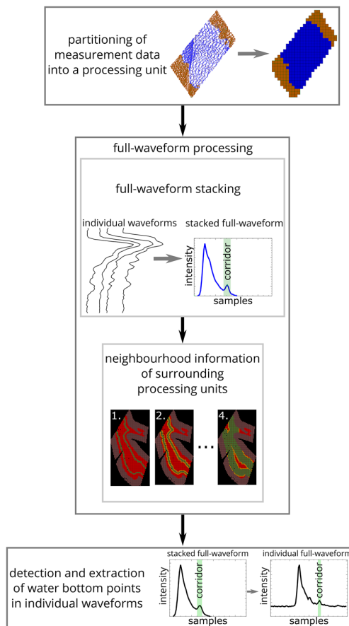
Fig. 4 Workflow of extended processing of full-waveform data
