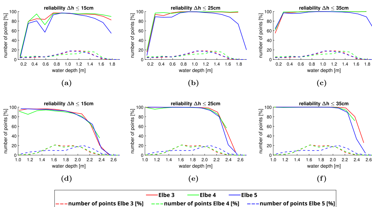
Fig. 16 Inlier rates in regard to their water depths of the comparison from the FWSP to (a–c) OWP points and (d–f) ES points
