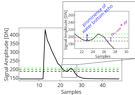
Figure 15: Application of multiple noise ranges ( n_{nr\_ampl} =factor) for checking the reliability of the water bottom echo. Black dashed line = amplitude of local minimum. Red dashed line = amplitude threshold ( n_{nr\_ampl} \cdot nr ). Green dashed line = amplitude of the water bottom peak.
