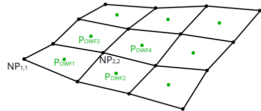
Figure 17: Calculating node points (black points) from ortho full-waveform analysis results (green points).
