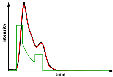
Figure 3. Schematic representation of SVB algorithm; green: dBCS model; red: model of the received signal; black: received signal.
