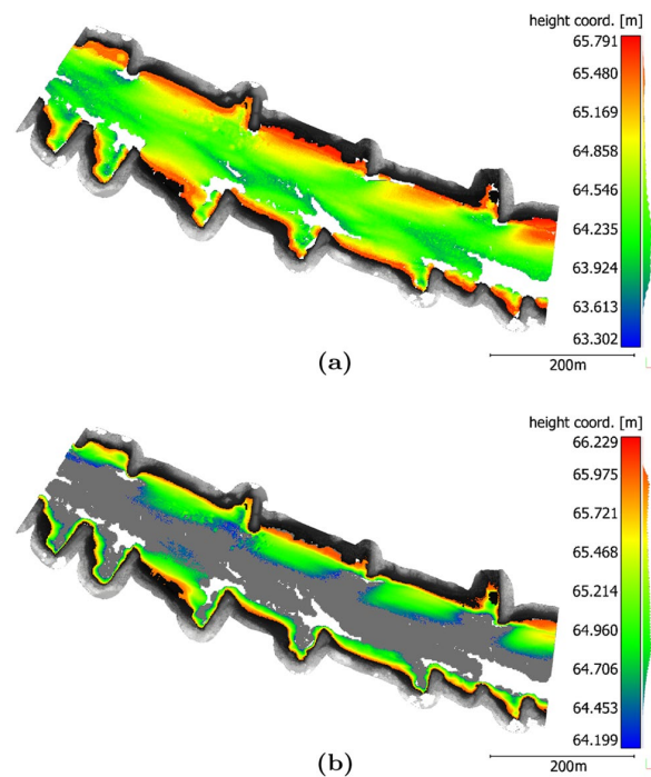
Fig. 10 Results of full-waveform stacking for investigation area Elbe 3. a The FWSP points are colour-coded corresponding to their height component (z-coordinate). b Illustration of the improved coverage of the riverbed by FWSP point cloud (dark grey). The OWP points are presented colour-coded corresponding to their height coordinate
