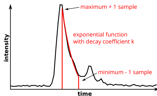
Figure 2. Schematic representation of volume backscatter extraction and exponential function approximation.
