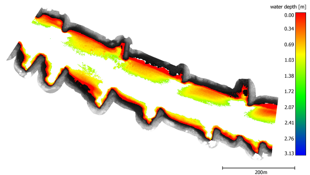
Figure 3: The online processed data of the investigation area are color-coded according to their water depth. Land points = gray.
