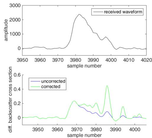
Figure 12. Recorded waveform (top), differential backscatter cross section (bottom blue) and attenuation-corrected differential backscatter cross section (bottom green) (Richter et al., 2017).
