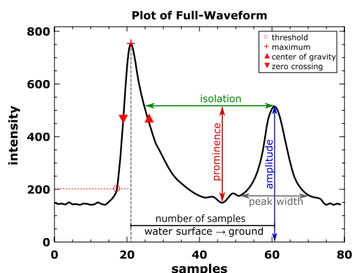
Fig. 5 Schematic representation of the parameter of a full-waveform analysis
