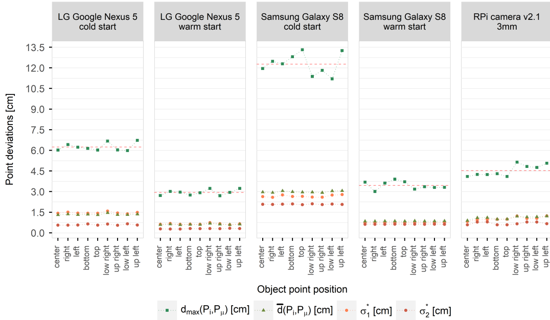
Figure (7.11): Principal standard deviations \sigma_1^* and \sigma_2^* giving the directional error in object space for each projected object point and for each investigated camera.
