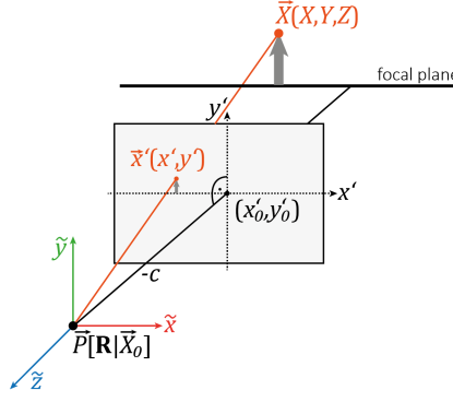
Figure (7.1): Transformation of a 3D object point \vec{X} into a 2D image point \vec{x}' where \vec{P}[\mathbf{R}|\vec{X}_0] is the camera projection center in a world coordinate system.
