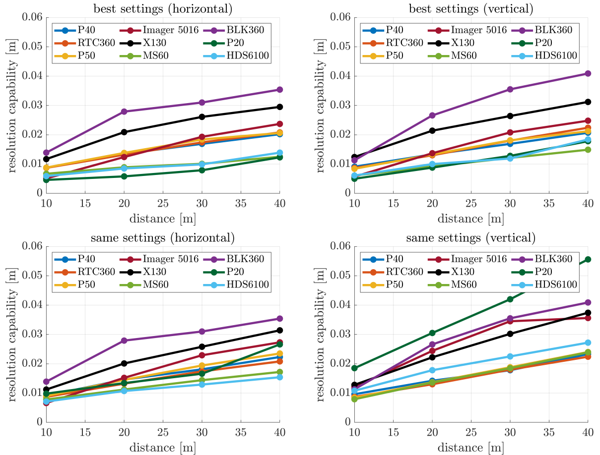
Abbildung 5.4: Resolution capability of different scanners at different distances; left: horizontal direction; right: vertical direction; top: best possible settings; bottom: almost same settings (modified from Schmitz et al. [2021a]).
