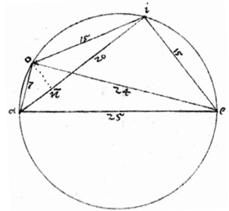
Abb. 27: Blatt 24r. Additionstheorem.
