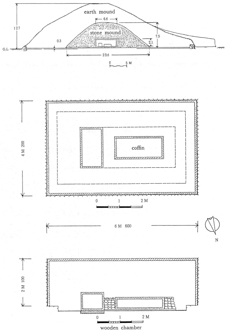
Section of Tomb 155 and section and plan of its wooden burial chamber
