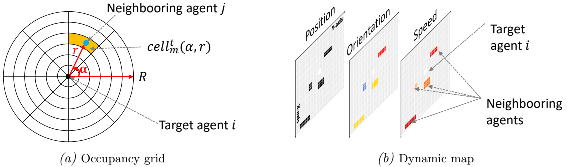
Figure 4.3: Agent-to-agent interaction modeled via occupancy grid and dynamic map at each step.
