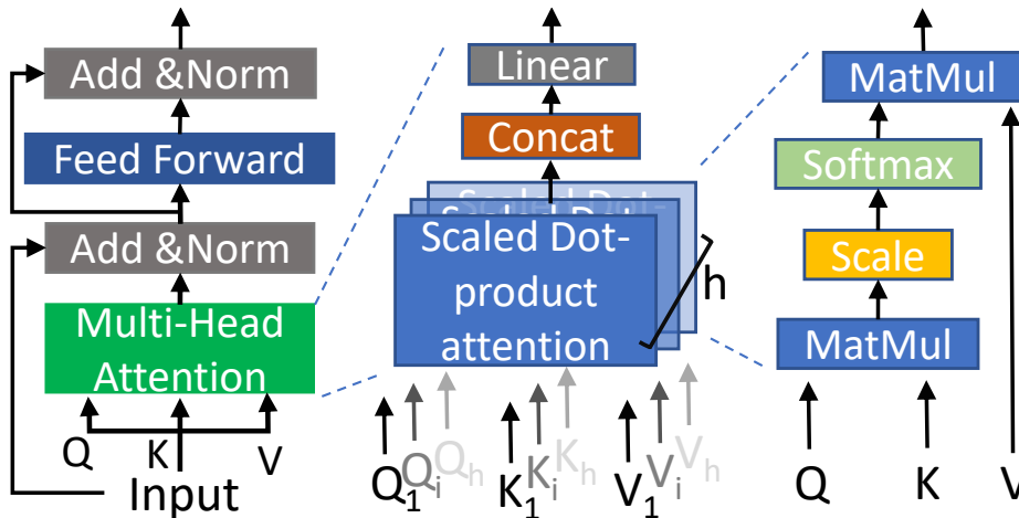
Figure 2.6: The Transformer encoder with a self-attention mechanism. Add stands for adding an identity mapping using a shortcut connection (He et al., 2016), Norm for layer normalization (Ba et al., 2016), Feed Forward for a feed-forward network, Concat for concatenation, and MatMul for matrix multiplication.
