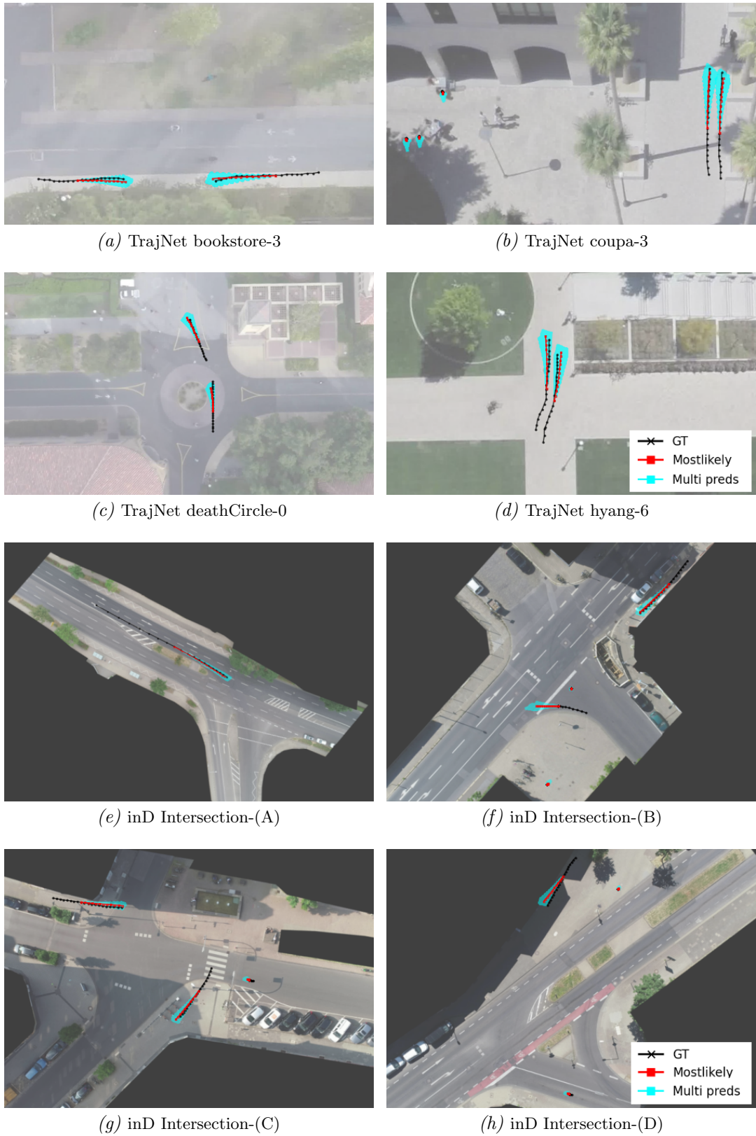
Figure 6.14: The qualitative results of DCENet. Multi-path trajectory predictions are generated by DCENet in the shared spaces of the TrajNet benchmark and at different intersections of the inD benchmark. The background images of (a)-(d) are retrieved from (Sadeghian et al., 2018a) and (e)-(h) are retrieved from (Bock et al., 2019).
