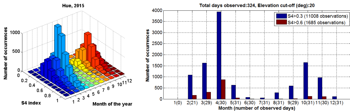
Figure 4.8b. Seasonal frequency of scintillation events appearance at HUE in 2015
