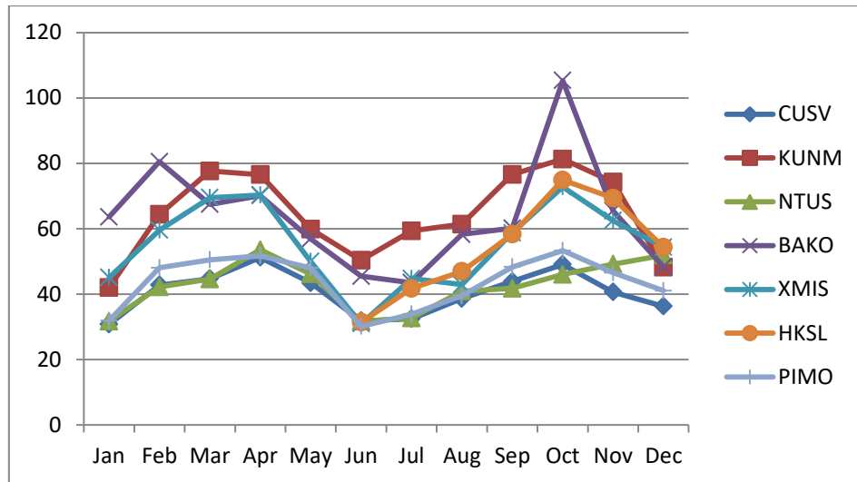
Figure 3.10a. Seasonal variations of the monthly maximum VTEC in 2010
