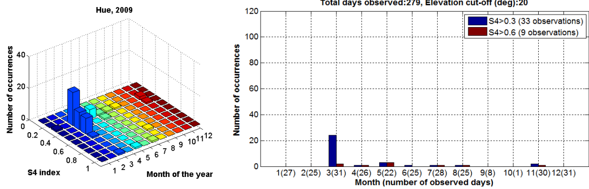
Figure 4.7b. Seasonal frequency of scintillation events appearance at HUE in 2009
