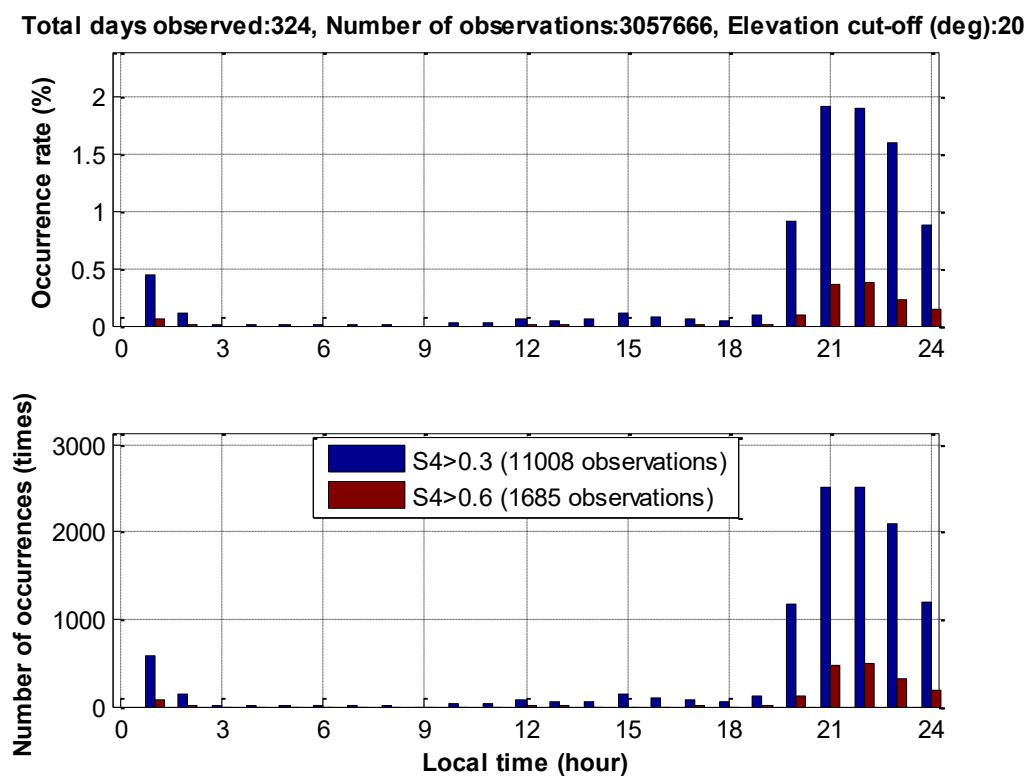
Figure 4.6b. Local time frequency of scintillation events appearance at HUE in 2015
