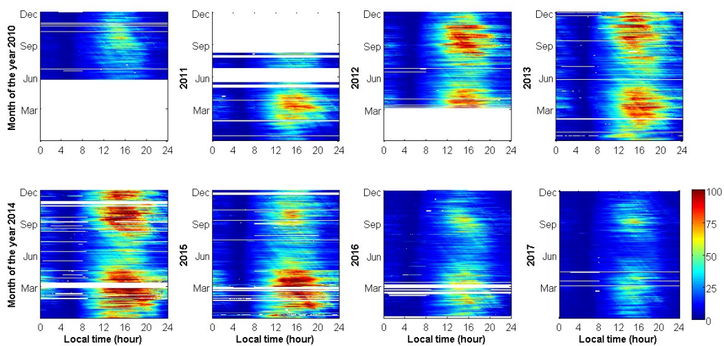
Figure 3.14f. VTEC map at station HKSL during SC24
