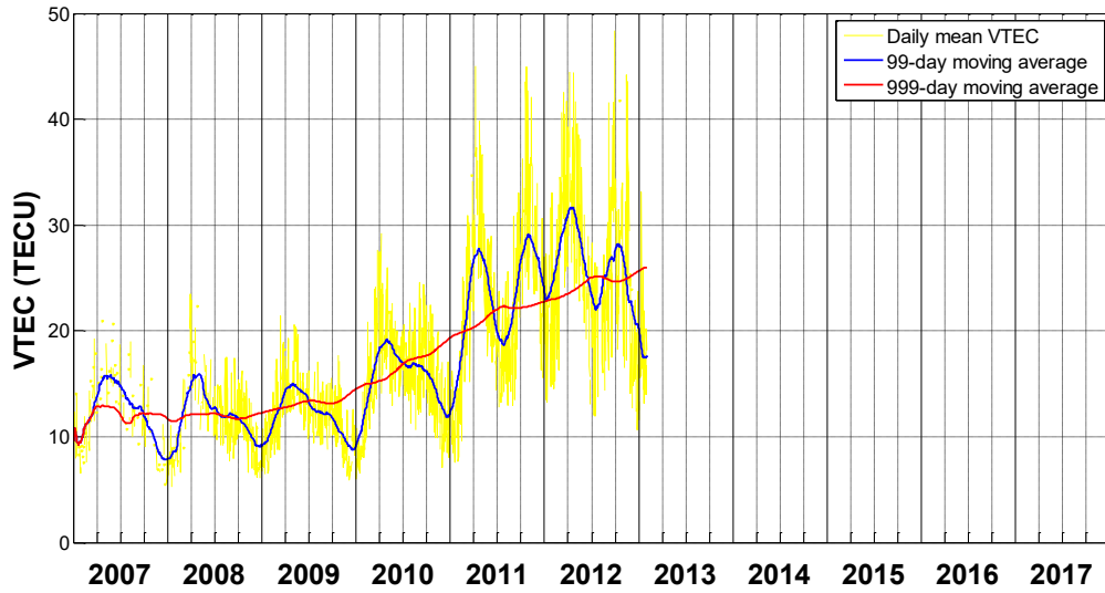
Figure 3.11g. Daily mean VTEC during SC24 at station KUNM
