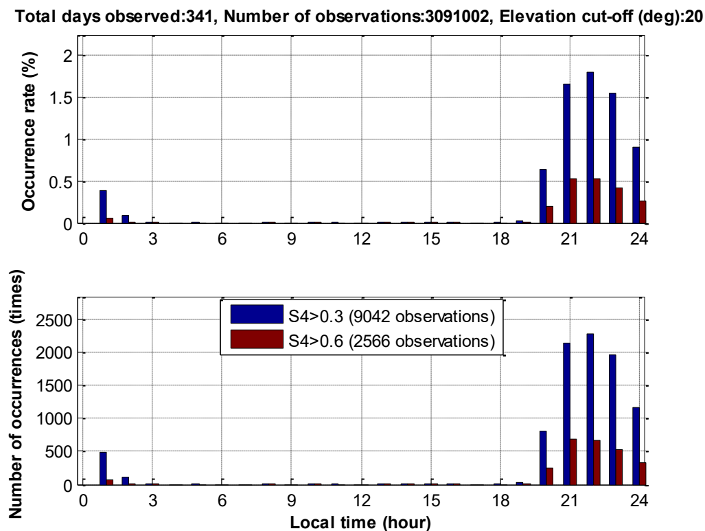
Figure 4.6a. Local time frequency of scintillation events appearance at HANOI in 2015
