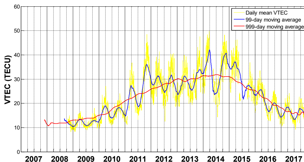
Figure 3.11d. Daily mean VTEC during SC24 at station CUSV
