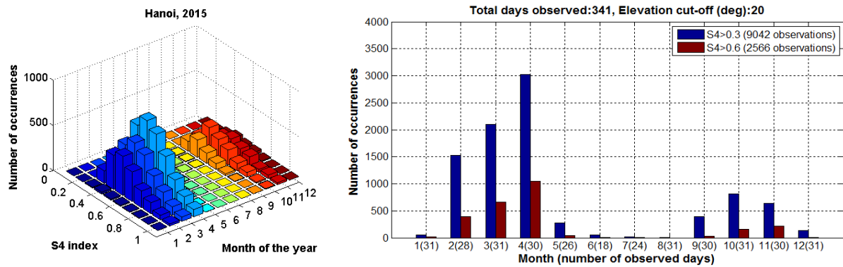
Figure 4.8a. Seasonal frequency of scintillation events appearance at HANOI in 2015
