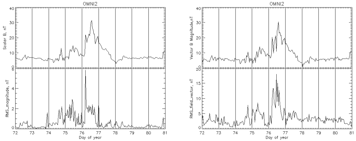
Figure 6.6a. Magnetic field indices during the middle of March 2015
