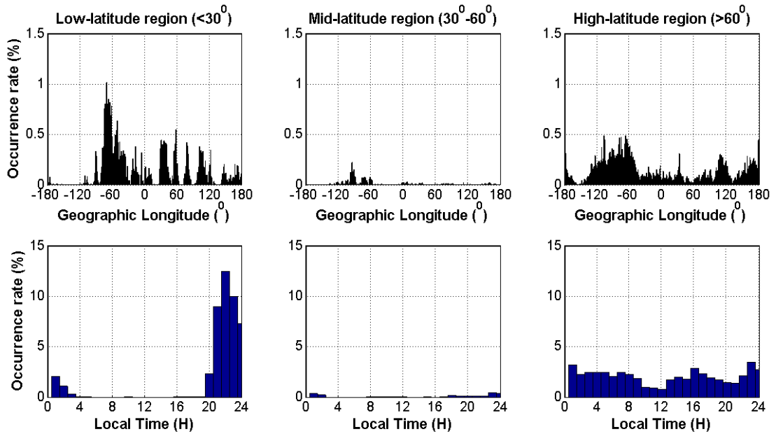
Figure 5.8d. Distribution of ROTI by longitude (above) and by time (below) at three different zones of the Earth (only ROTI ≥ 0.5 TECU/min are counted). While the mid-latitude areas show almost nothing as can be predicted, the high-latitudes are the regions where ionospheric irregularities can occur randomly at any longitude and at any time of the day. The appearance rule is most straightforward in the low-latitude regions with the appearing time only at night and most concentrated in the area of 60°W longitude (the South America region).
