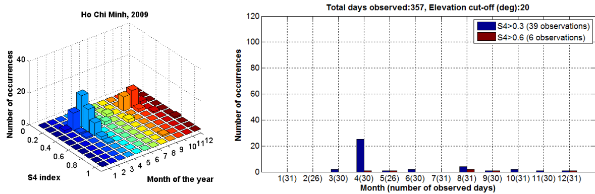
Figure 4.7c. Seasonal frequency of scintillation events appearance at HCM in 2009
