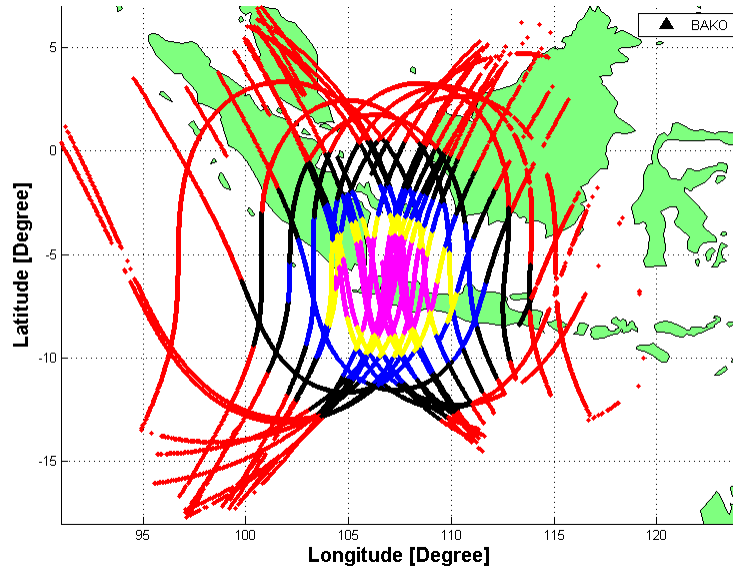
Figure 2.3. The footprint of satellite tracks at BAKO station in a single day. Different colors correspond to different satellite elevations: [0:20^\circ] : red, [20^\circ-30^\circ] : black, [30^\circ-40^\circ] : blue, [40^\circ-50^\circ] : yellow and [50^\circ-90^\circ] : magenta.
