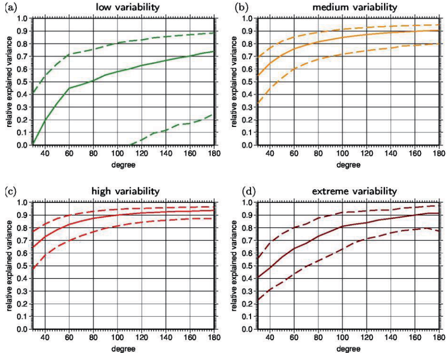
Figure 3.1-7: Quantiles (25%, 50%, 75%) of the relative explained variances for 1° continental grid boxes of the updated ESA Earth System Model for different cutoff degrees of the spherical harmonic expansion. 1° Grid boxes were grouped into for classes of different de-trended and de-seasonalized daily storage variability, i.e. of 0.5 - 3 cm (a), 3 - 7 cm (b), 7 - 20 cm (c), and > 20 cm (d).
