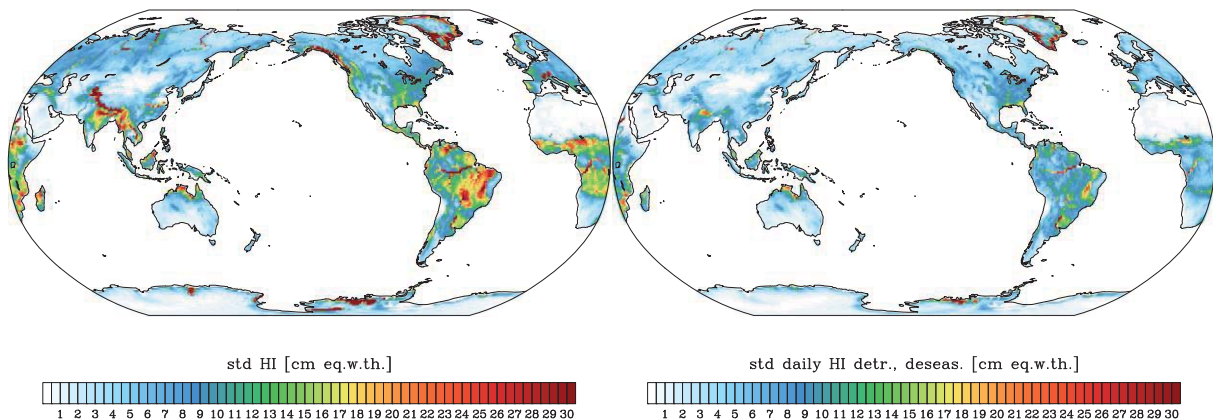
Figure 3.1-5: Standard deviation of 12 years of daily terrestrially stored water mass anomalies simulated by LSDM (Dill 2008) for the updated ESA Earth System Model (Dobslaw et al. 2015): full signal content (left) and after the removal of linear trend and annual cycle (right).
