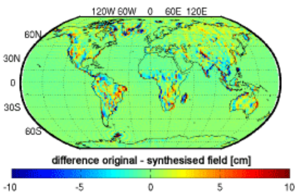
Fig. 2.3.3: Differences between water mass storage from ECOCTH and synthesized field from gravity field coefficients in April 1990 expressed in equivalent water heights.
