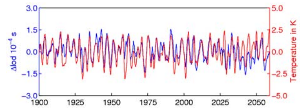
Fig. 3.1.7: Sea Surface Temperature (SST) in the Western Tropical Pacific and LOD. Blue line: The LOD variations induced by the oceanic matter term. Red line: Sea surface temperature anomalies in the Niño 3.4 region.
