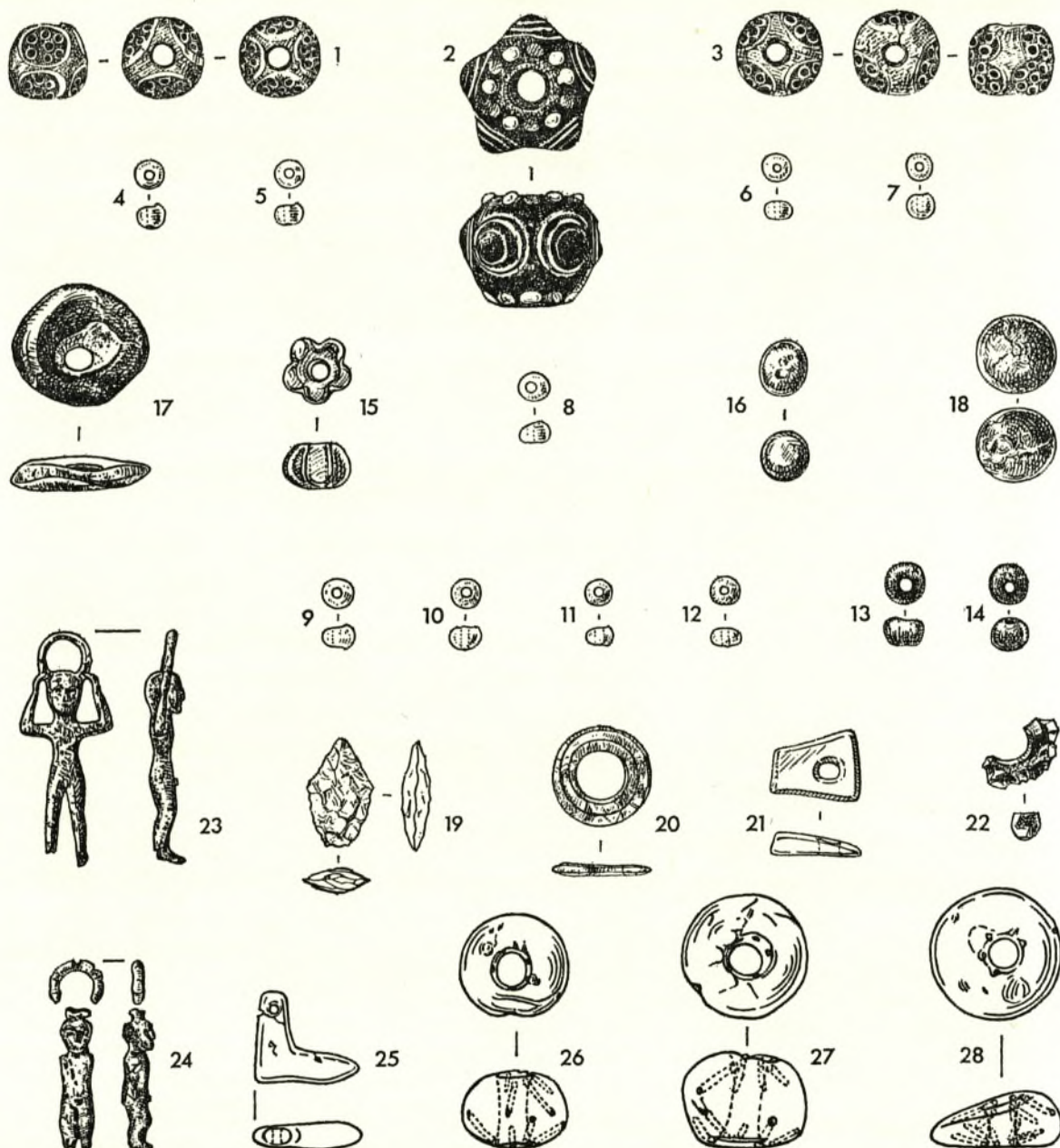
Abb. 17. Reinheim (96). — 1–15.20.22 Glas; 25–28 Bernstein; 16 Hornstein?; 17 Quarzit; 18 Jaspis; 19 Chalzedon; 23.24 Bronze. M. 1 : 2.
